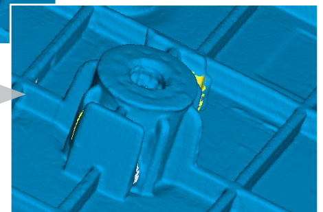
Triangle mesh from a 3D scanner with a resolution of 5 MP (Field of view 480x350 mm)
